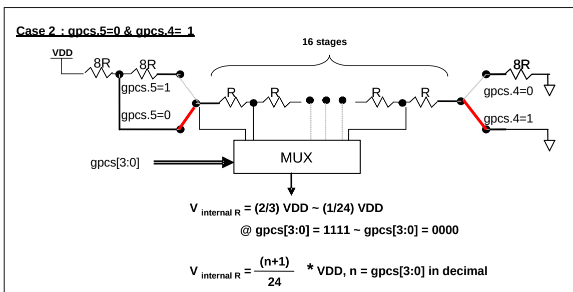
Fig. 6: V_{\text{internal R}} hardware connection if gpcs.5=0 and gpcs.4=1
