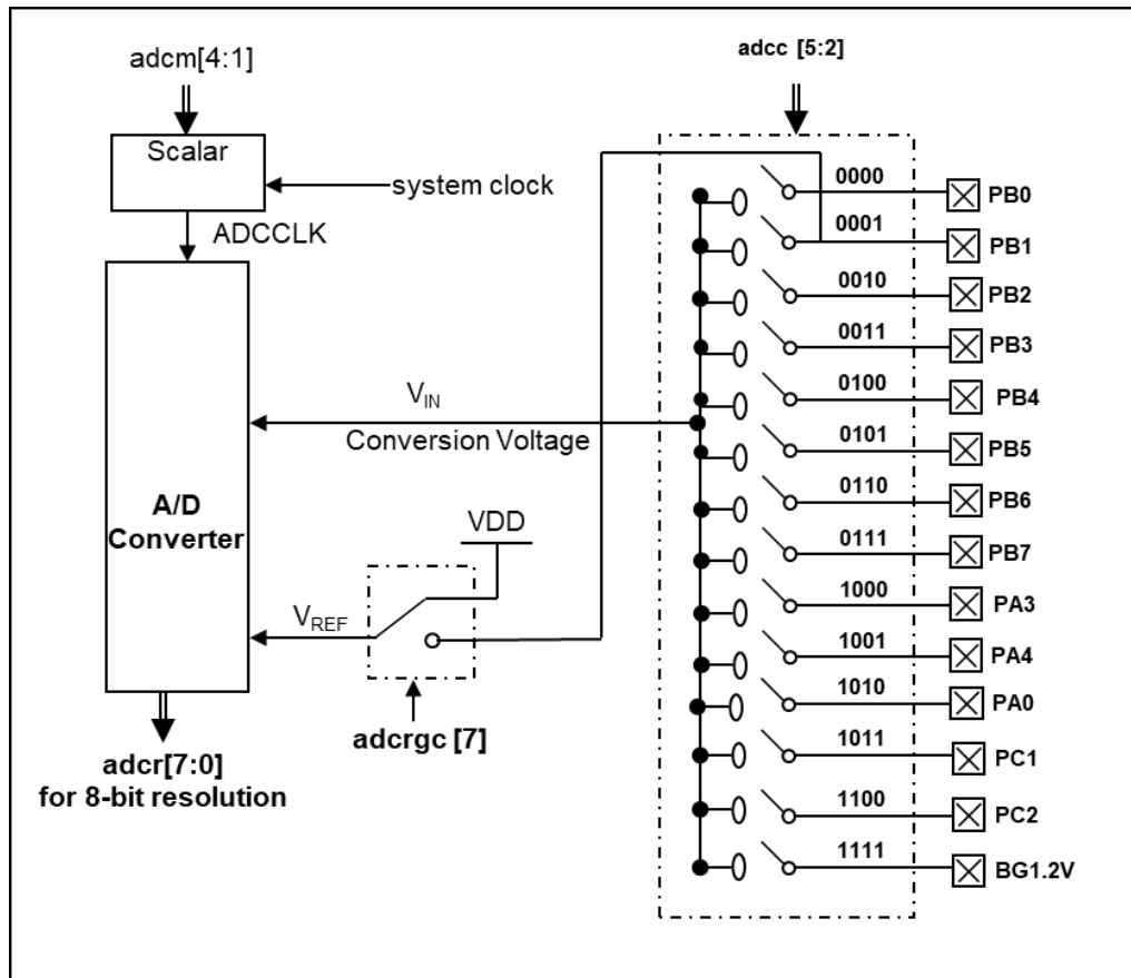
Fig. 20: ADC Block Diagram
