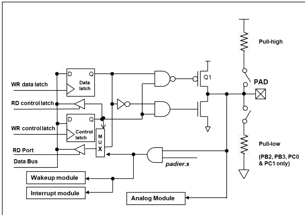
Fig. 19: Hardware diagram of IO buffer
