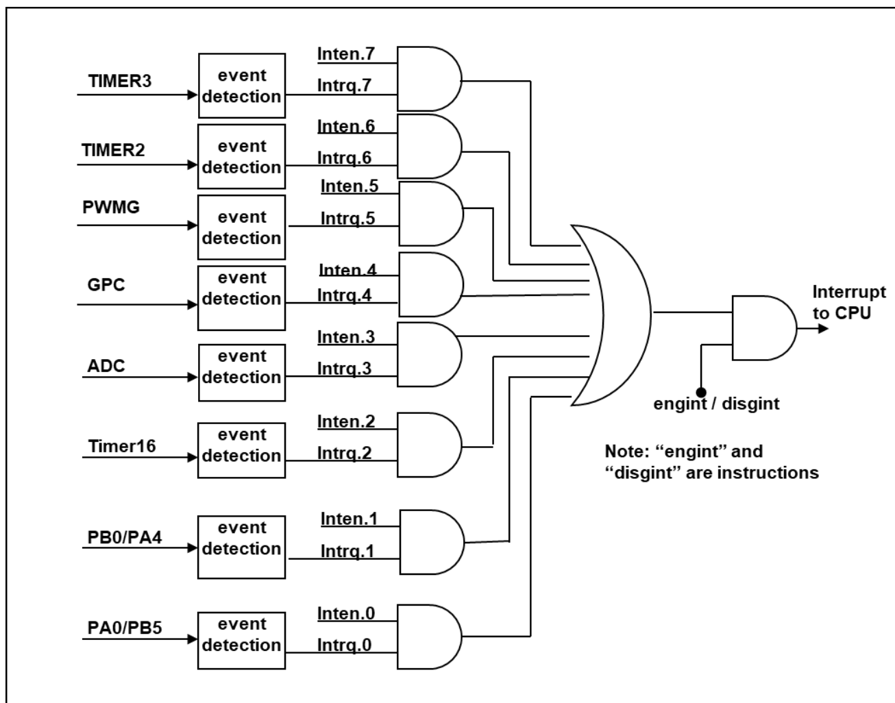
Fig.18: Hardware diagram of interrupt controller
